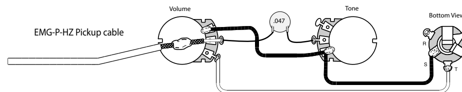
EMG-P-HZ Diagram 2 1 Volume, 1 Tone
