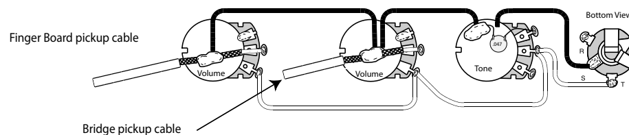
EMG-P-HZ Diagram 3 2 Volume, 1 Tone (each Volume is independent)
